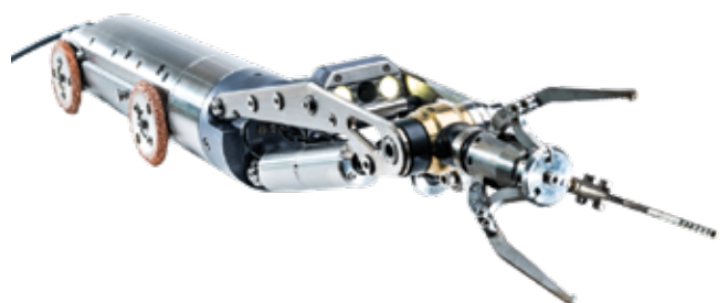
Solid Debris Removal Gripper
